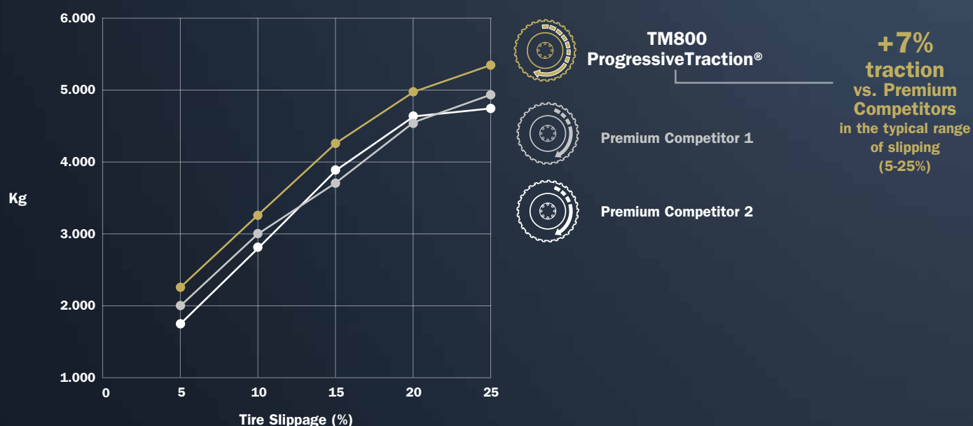
Traction force Higher is better
